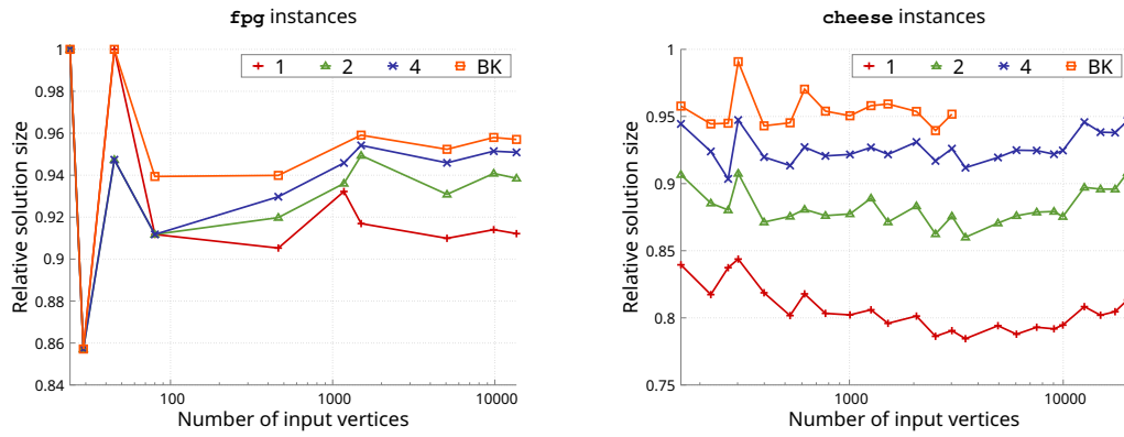
Figure 9 Solution sizes relative to the best Challenge solution. Data is based on a triangulation replicated 1, 2, or 4 times and randomly bloated using V . Alternatively, we use Bron-Kerbosch (BK) to obtain all V -maximal polygons, when the running time is not too long. Afterwards, all collections are bloated again using V \cup S_2(C) and solved using IP.
