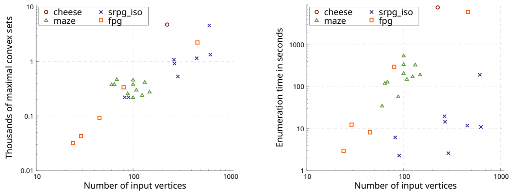
Figure 5 Number of (V \cup S_1) -maximal convex polygons and the time to enumerate them.
